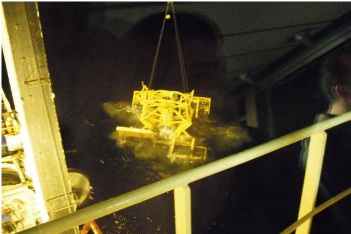
Installation of Fast Frame From the Deep Pioneer
